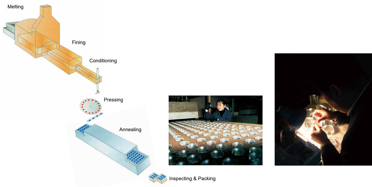
Main Process of Making Ophthalmic Lens Blanks
