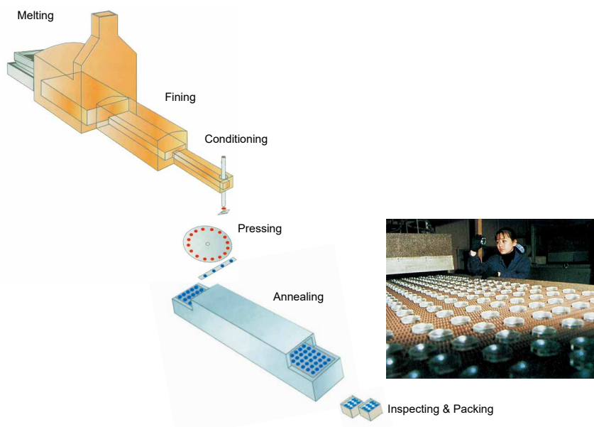
Main Process of Making Ophthalmic Lens Blanks
